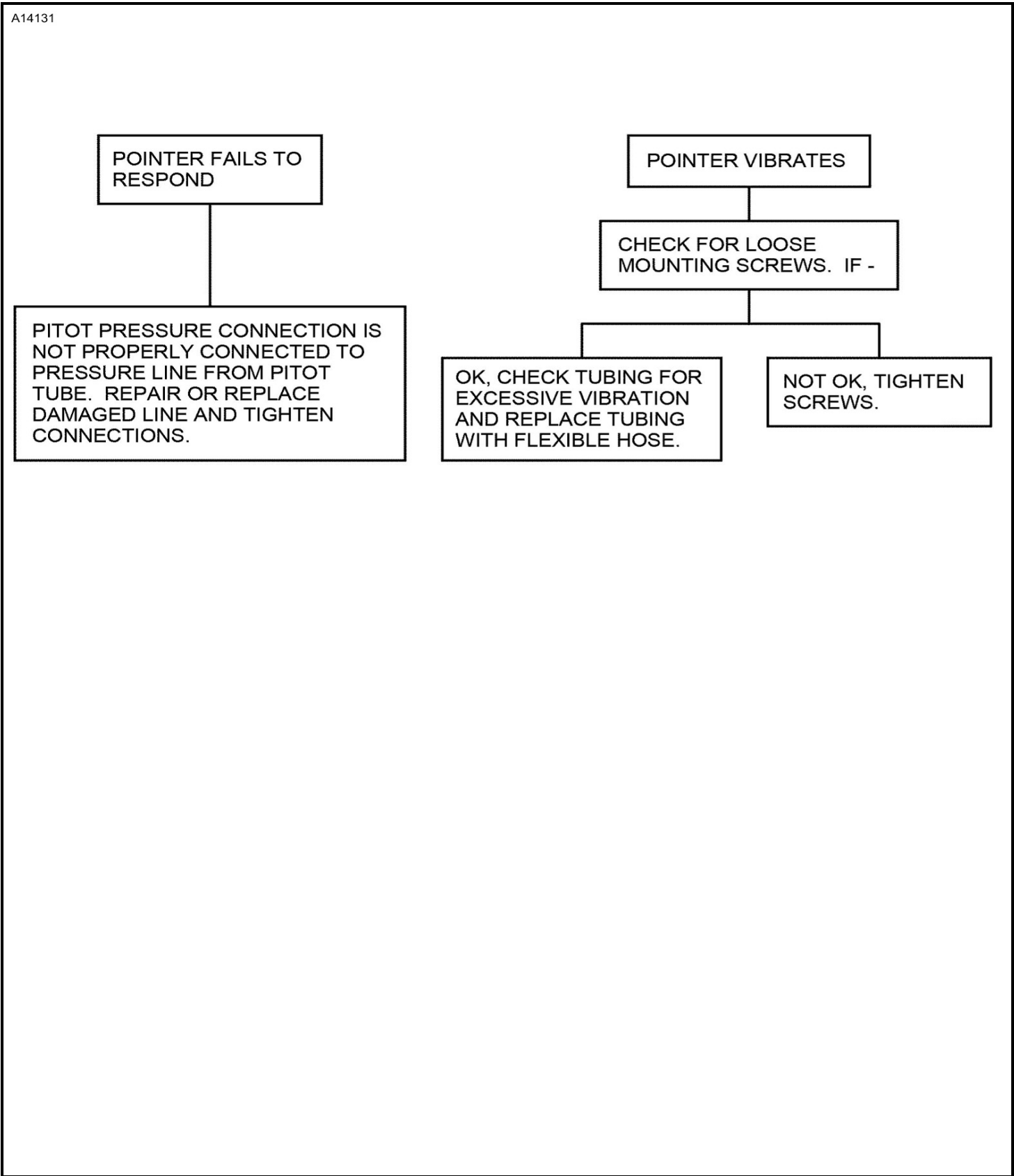
Figure 101 : Sheet 2 : Airspeed Indicator Troubleshooting Chart
